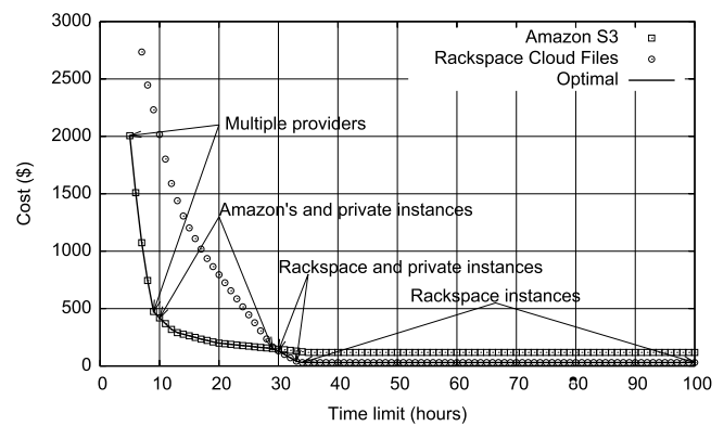
Fig. 6. Large data processed on finite public cloud.
