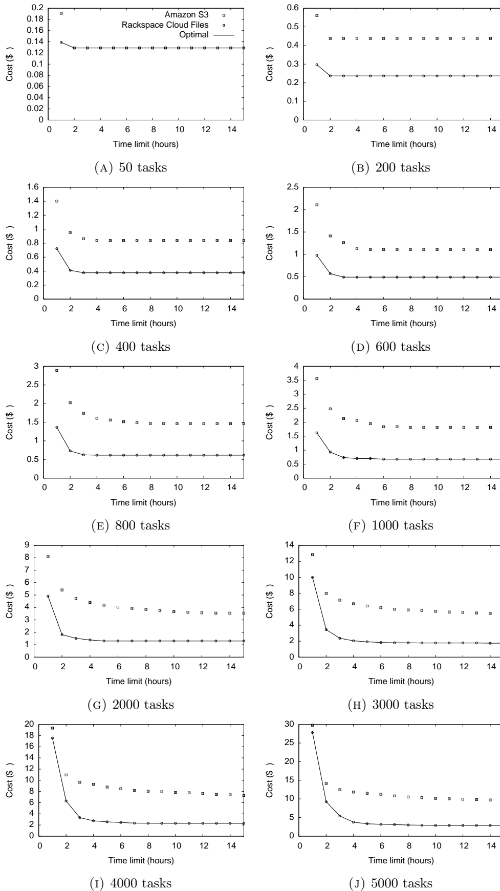
FIGURE 5.7: Optimal cost found by the model for SIPHT workflow.
