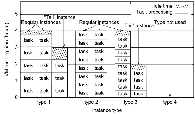
Fig. 2. Task scheduling policy.
